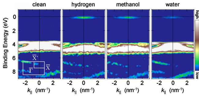
FIG. 2. (Color online) Intensity plots of the second derivatives of the ARPES spectra along the \Gamma\bar{X}' axis. The spectra were recorded with h\nu=65 eV. Bright regions correspond to the bands. The surface Brillouin zone of ZnO(10 \bar{1} 0) is displayed in the inset.
