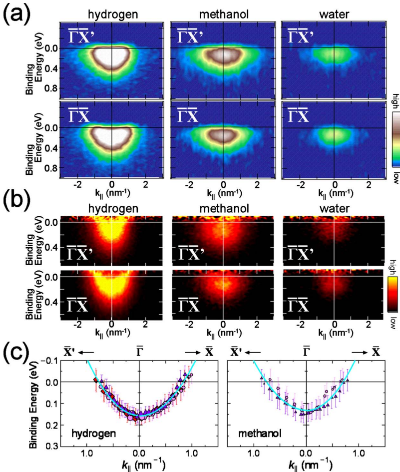
FIG. 3. (Color online) (a) ARPES-intensity plots of the adsorbate-induced bands along two high-symmetry axes. (b) Plots of the emission intensity divided by a Gaussian-convoluted FD function. (c) Plots of the peak positions in the ARPES spectra divided by a Gaussian-convoluted FD function. The results of independent measurements are shown by different symbols. The size of symbols represents the emission intensity of the peaks. Solid lines through the plotted symbols are fitted results by parabolas assuming parabolic energy dispersion of the metallic bands.
