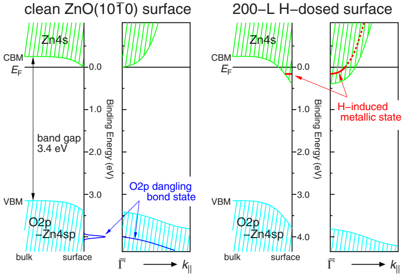
FIG. 4. (Color online) Schematic of the energy band structures of the clean and H-covered ZnO(10 \bar{1} 0) surfaces. Essentially the same mechanism should be operative for the methanol- and water-adsorption systems but with a lesser extent of induced downward band bending.
